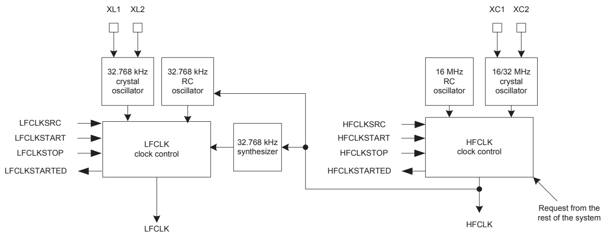
Figure 5 Clock management
