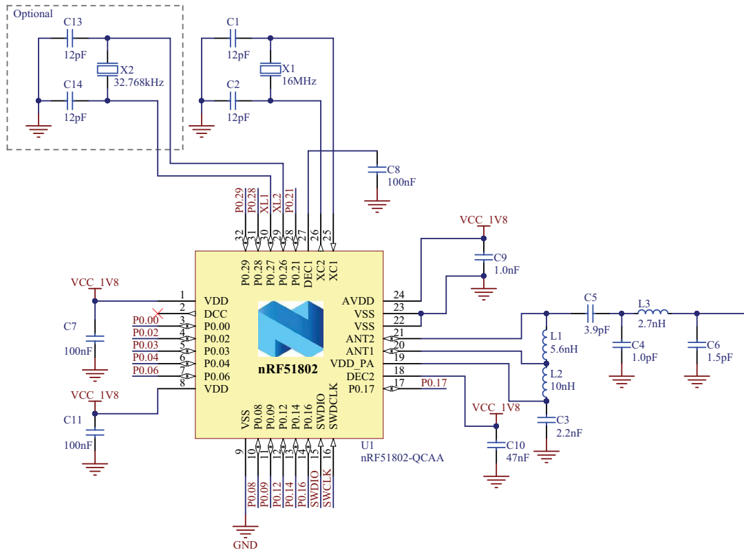
Figure 23 QCAA QFN32 with low voltage mode setup
