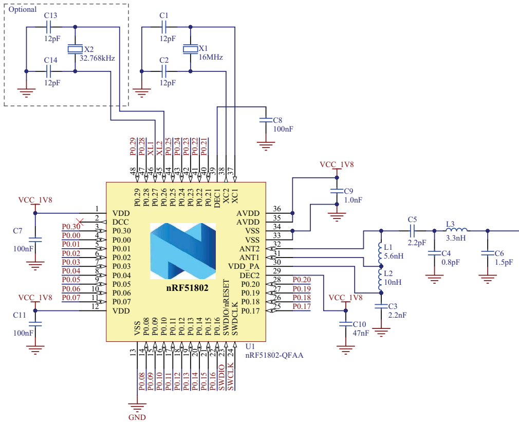
Figure 20 QFAA QFN48 with low voltage mode setup
