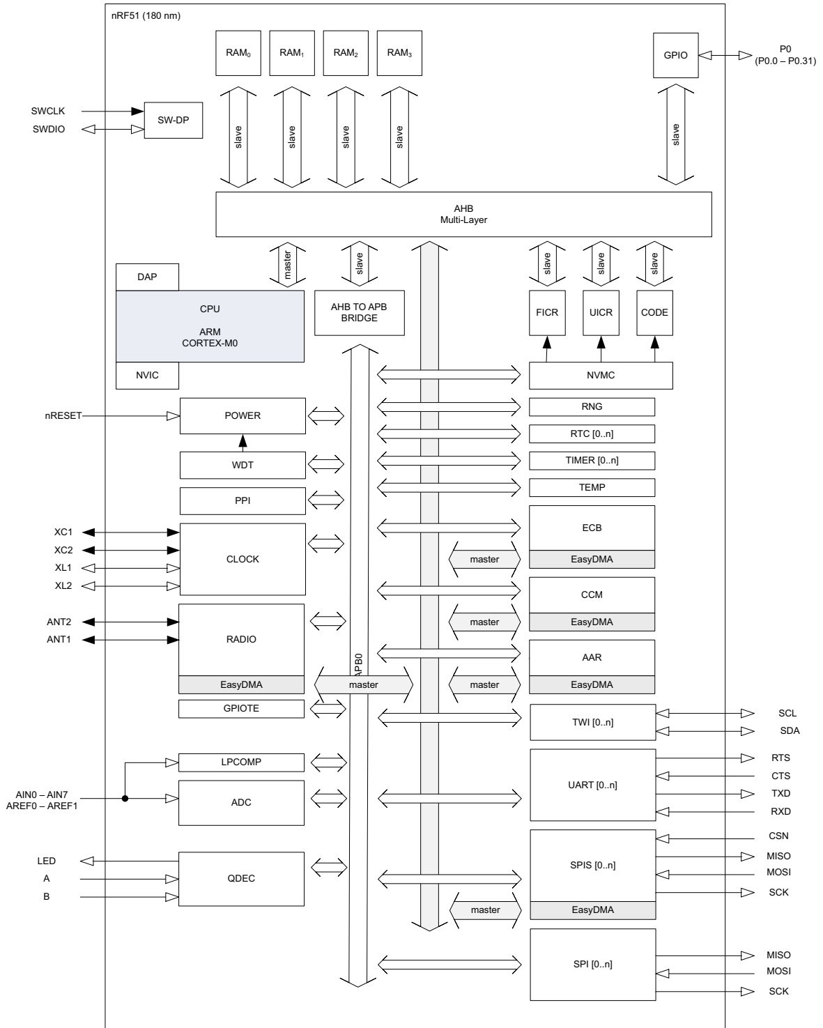
Figure 1 Block diagram
