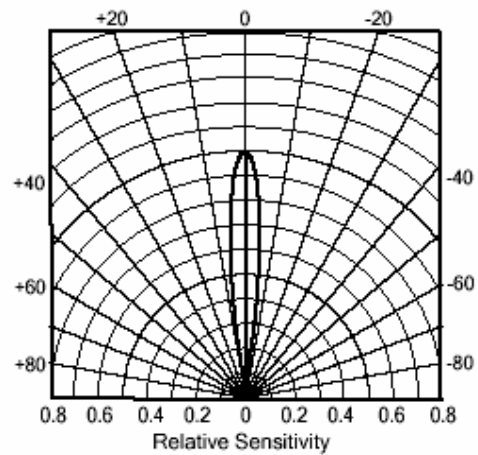
● Directive Characteristics
